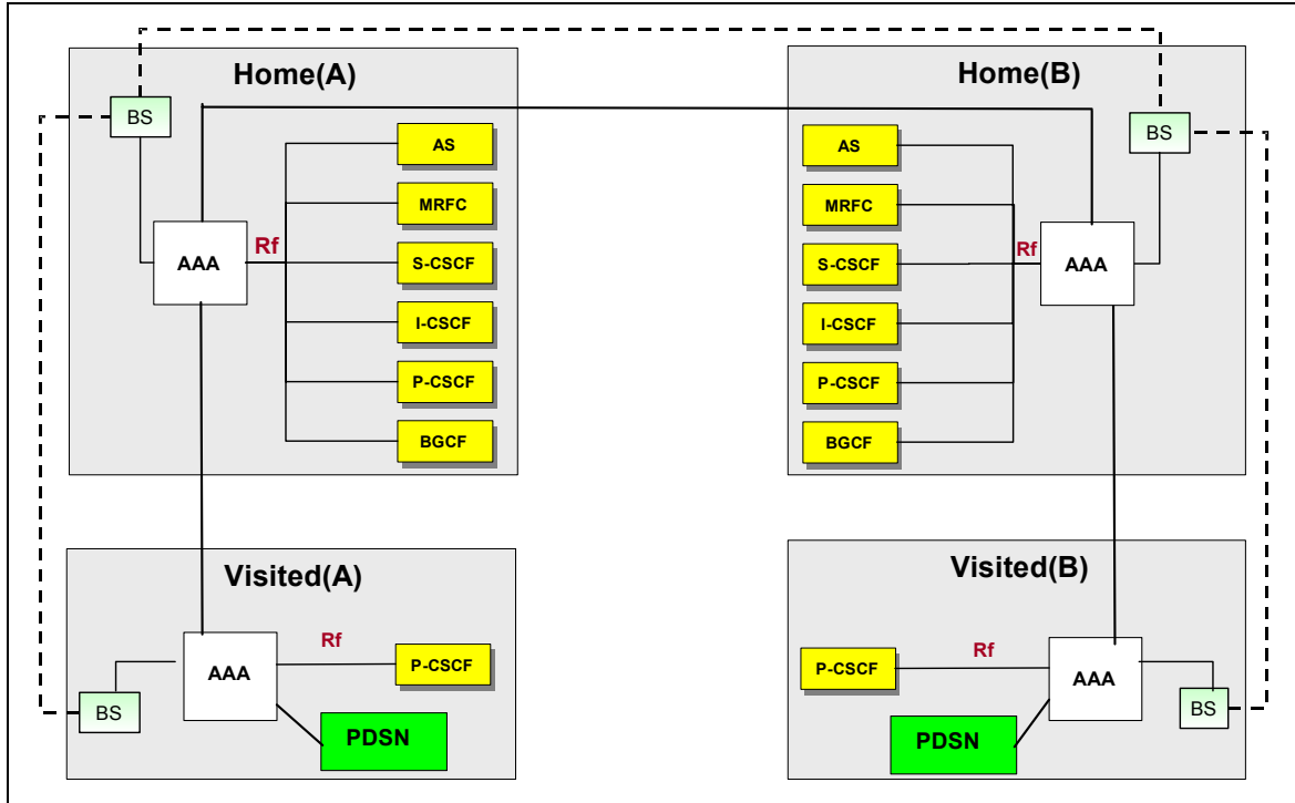
Figure 4.3: Off-line IMS Charging architecture for roaming scenario
