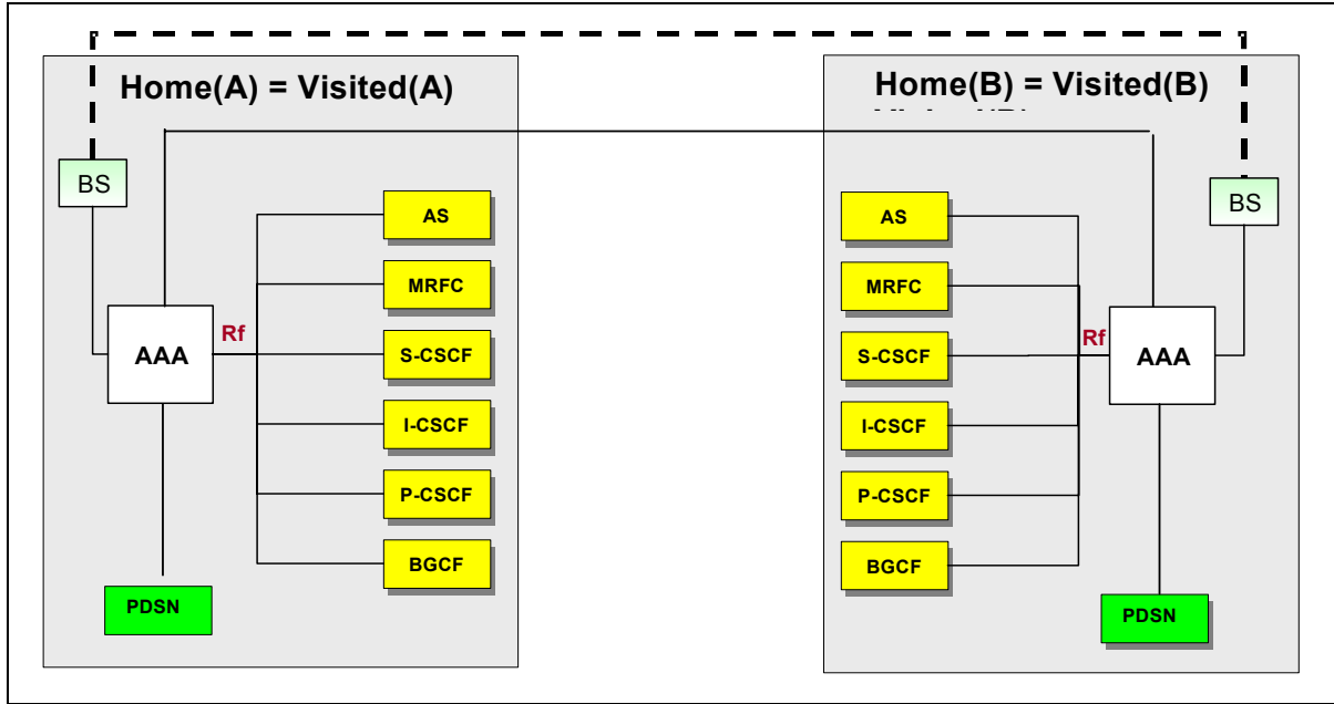
Figure 4.2: Off-line IMS Charging architecture for non-roaming scenario
