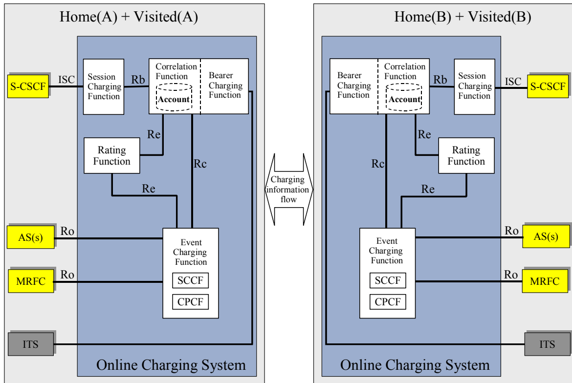
3 Figure 4.4: On-line IMS Charging architecture
