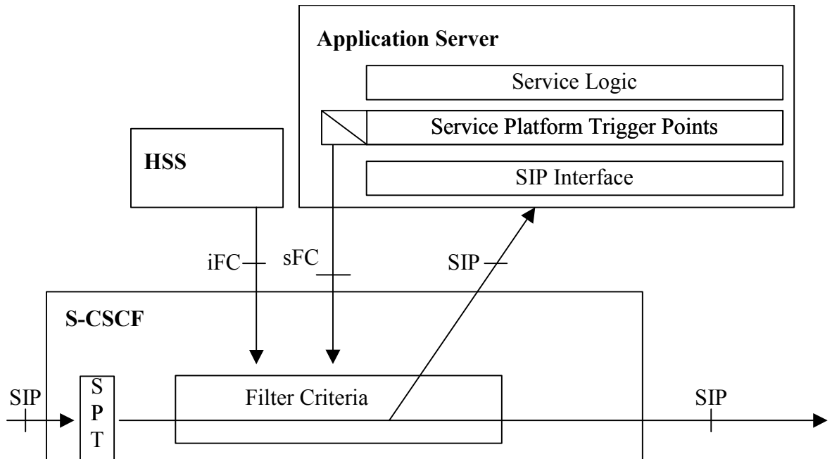
17 18 19 Figure 5.2.1: Application triggering architecture
