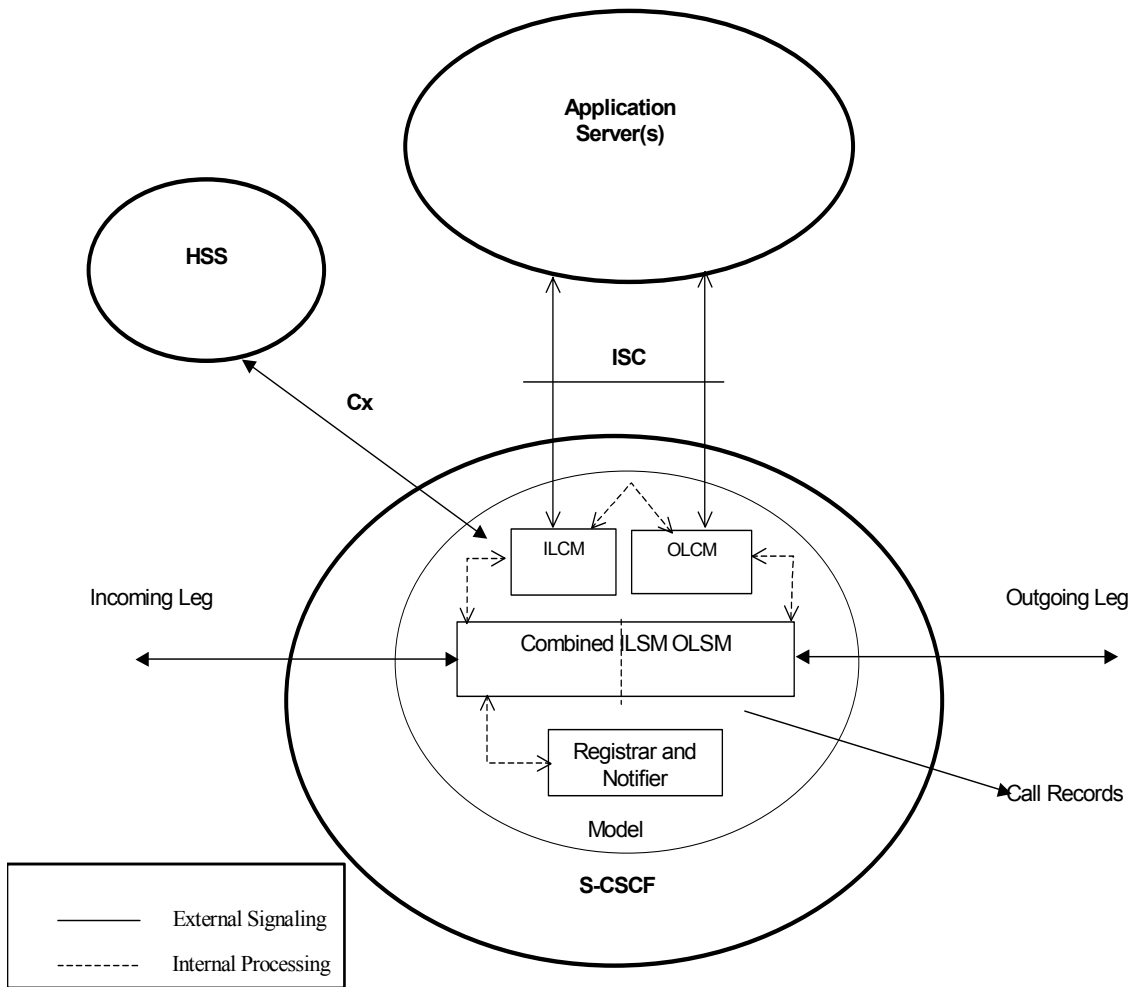
14 Figure 6.1.1.1: S-CSCF functional model with incoming leg control and outgoing leg 15 control
