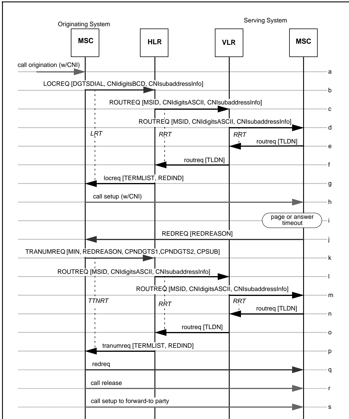
Figure 6 — CNIP Invocation to a Forwarded-To Subscriber
