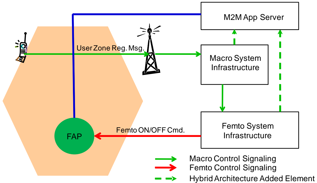
Figure 4.5-5: Hybrid Architecture
