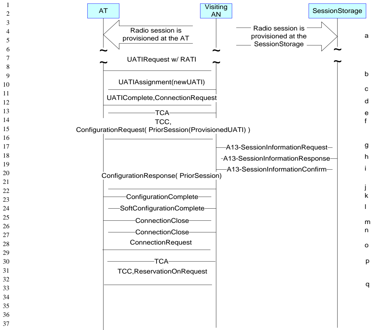
Figure 9-1 PriorSession retrieval when PriorSessionGAUP not supported
