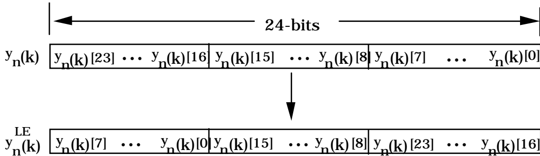
Figure 2. Reshuffling of y_n(k) to Generate y_n^{LE}(k)
