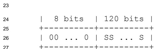
28 Figure 2.9.2.1.2-3. “S” bits in the Reserved IPv6 Address Format
