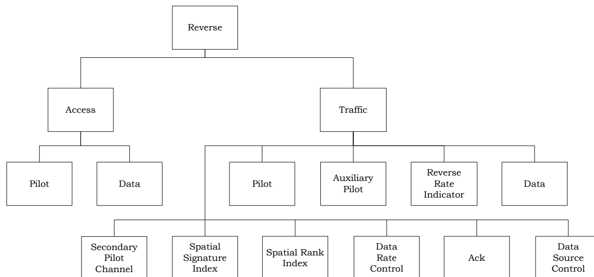
5 Figure 1.5-2. Reverse Channel Structure
