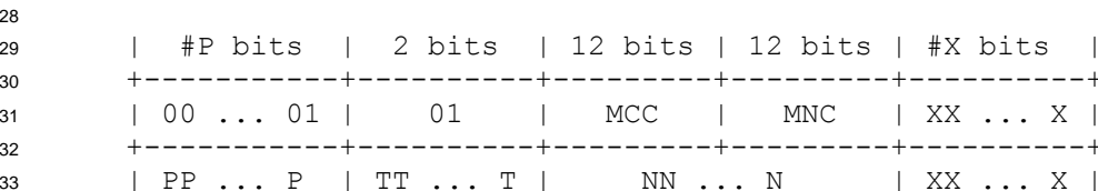
34 Figure 2.9.2.1.2.2-1. Assignment of the “T” Bits, the “N” Bits, and the “X” Bits for 35 the GSM/UMTS Method
