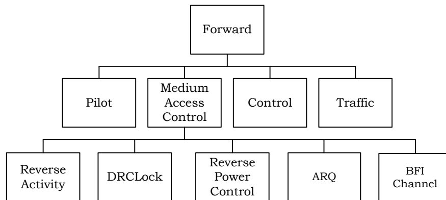
29 30 Figure 1.5-1. Forward Channel Structure
