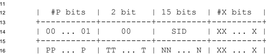
17 Figure 2.9.2.1.2.1-1. Assignment of the “T” Bits, the “N” Bits, and the “X” Bits for 18 the ANSI-41 Method
