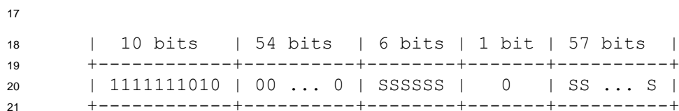
22 Figure 2.9.2.1.2-2. “S” bits in the Link-Local Unicast IPv6 Address Format
