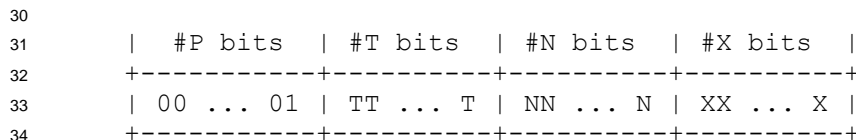
35 Figure 2.9.2.1.2-4. sub-fields of the “S” bits
