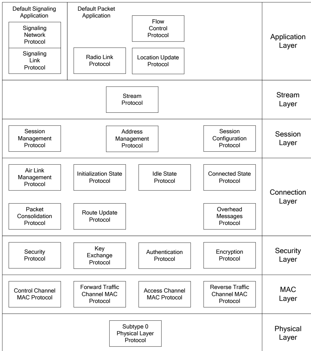
Figure 1.6.6-1. Default Protocols
