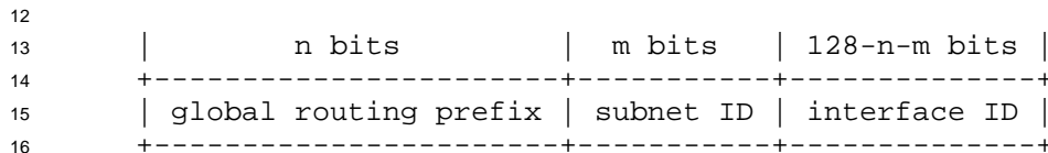
Figure 2.9.1.1-1. Global Unicast IPv6 Address Format
