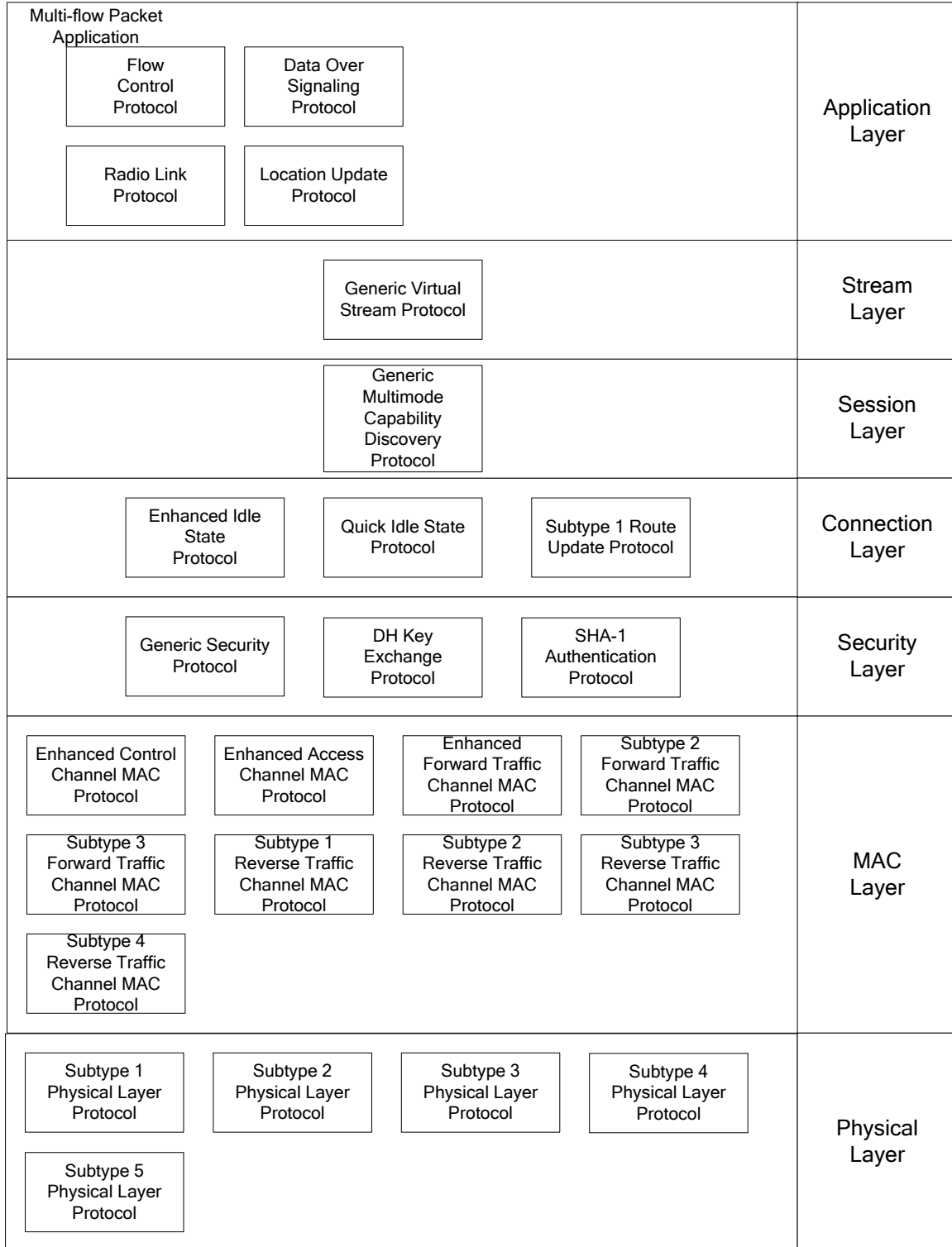
Figure 1.6.6-2. Non-Default Protocols
