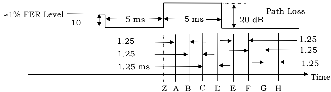
Figure 4.2.3.2-2. Path Loss Increase and Decrease Responses and the Test Points for the Alternative Test Procedure
