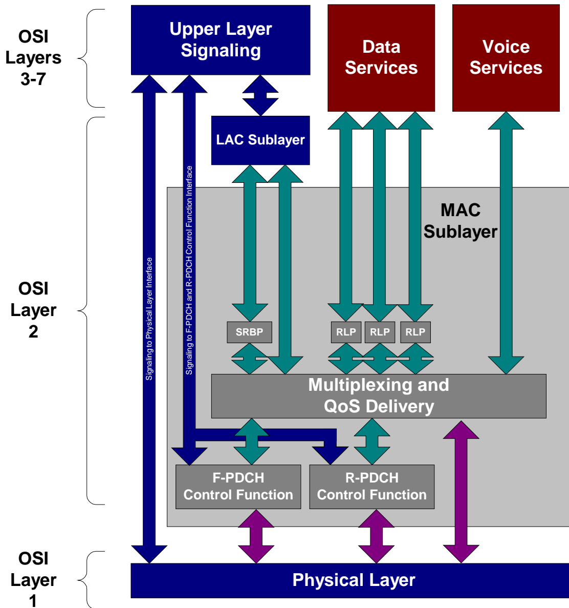
Figure 1 cdma2000 Architecture
