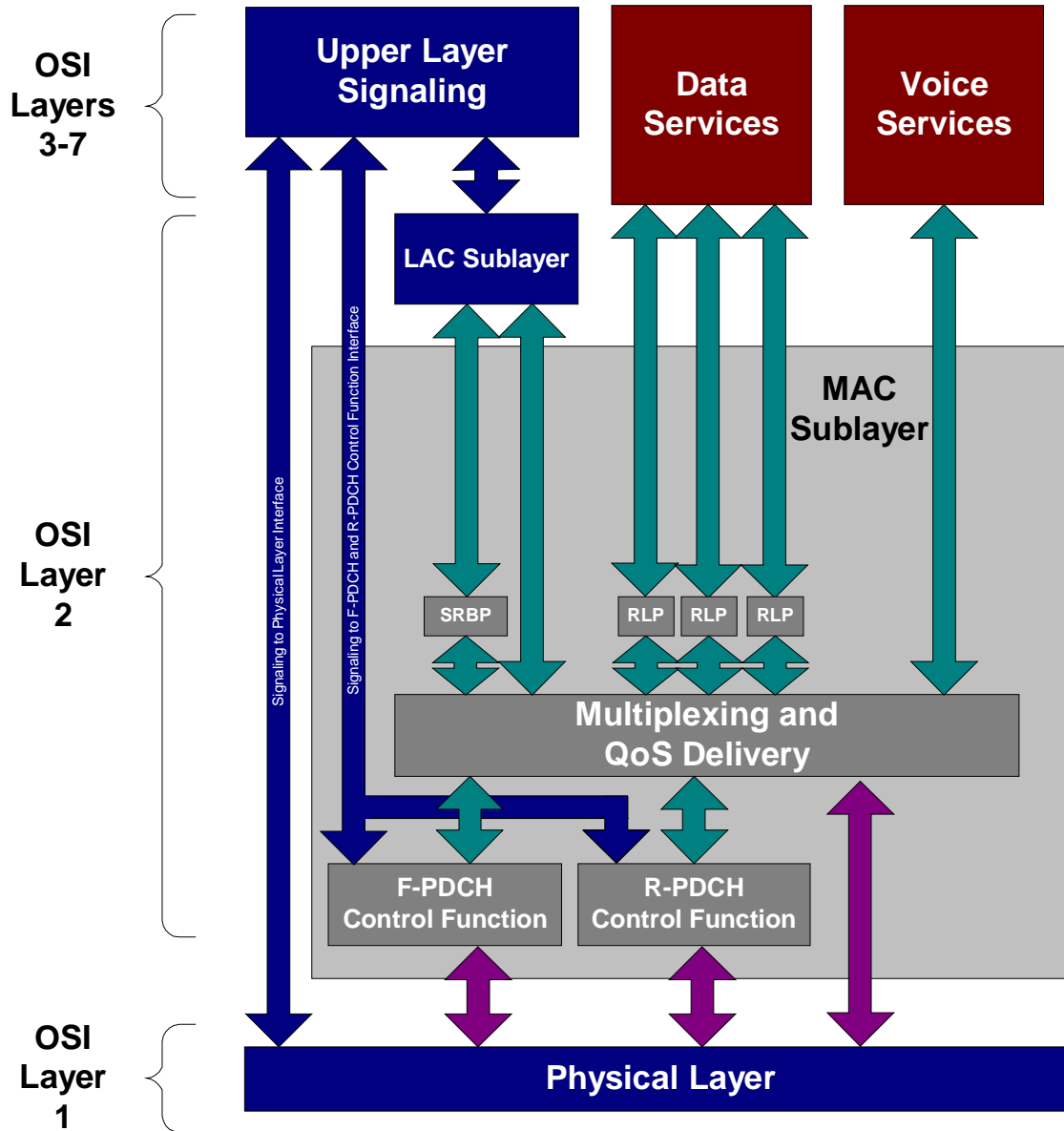
Figure 1 cdma2000 Architecture
