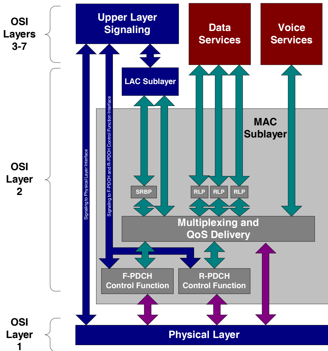
8 Figure 1 cdma2000 Architecture
