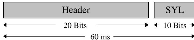
Figure B.12: Construction of the IS_SYL Message
