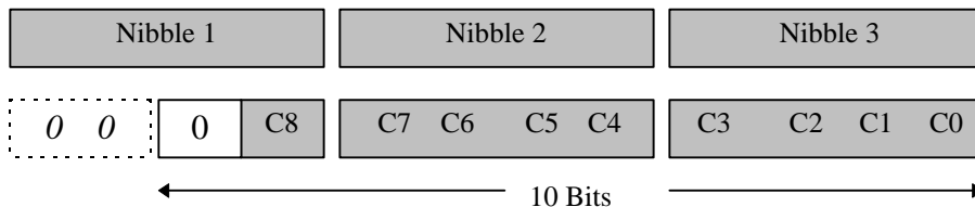
Figure B.4: General Construction of an IS_Command_Block
