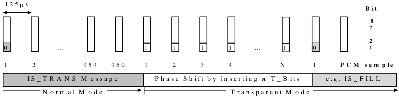
10 Figure B.14: Phase Shift of the 16_PCM_Sample_Grid by inserting T_Bits
