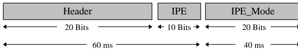
Figure B.8: General Construction of an IS_IPE Message
