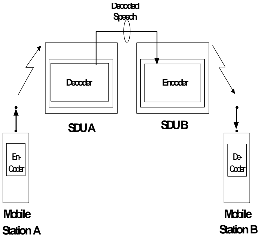
13 14 15 Figure A,.1: Logical Diagram of the Speech Path for Digital Calls 16 from Mobile A to Mobile B
