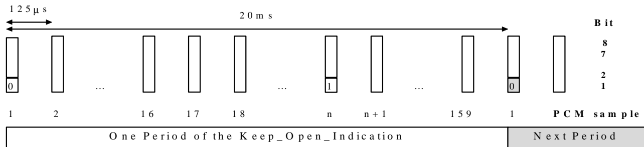
Figure B.13: Keep_Open_Indication
