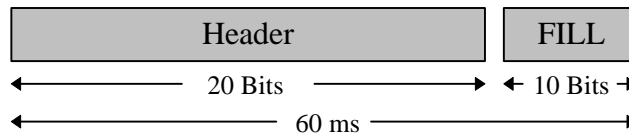
Figure B.10: Construction of the IS_FILL Message
