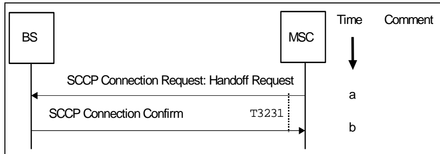
Figure 3.1.3.4.1.2-1 SCCP Connection Establishment During Handoff
