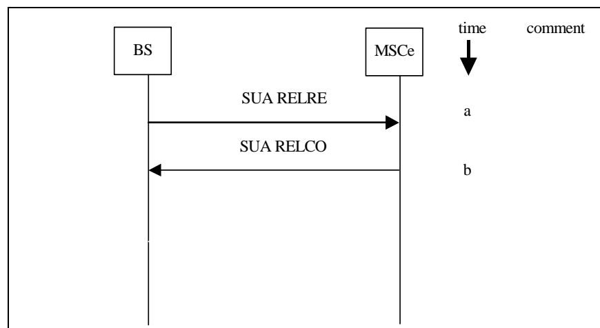
Figure 3.2.2.6.3.1-1 BS Initiated SUA Release: BS Lost SUA Connection Information
