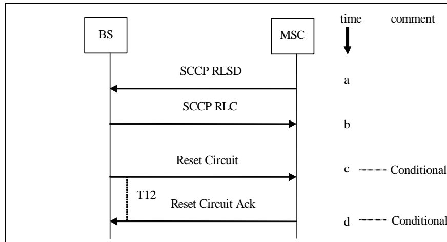
18 Figure 3.1.3.4.3.2-1 MSC Initiated SCCP Release: MSC Lost SCCP Connection Information
