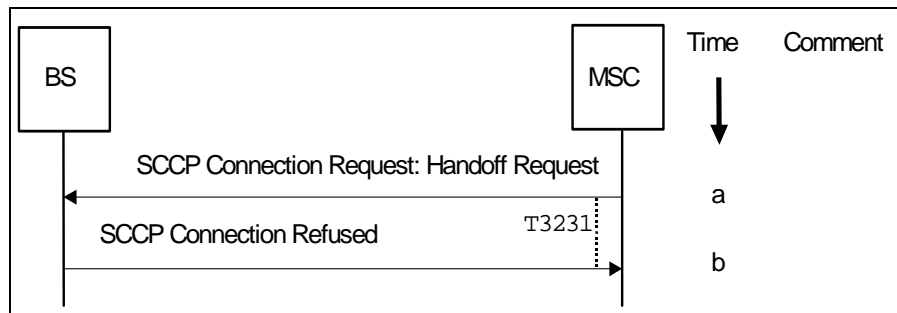
Figure 3.1.3.4.1.2-2 SCCP Connection Refusal During Handoff
