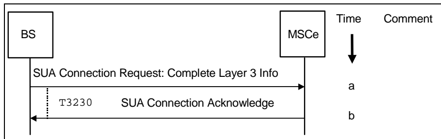
30 Figure 3.2.2.6.1.1-1 SUA Connection Establishment
