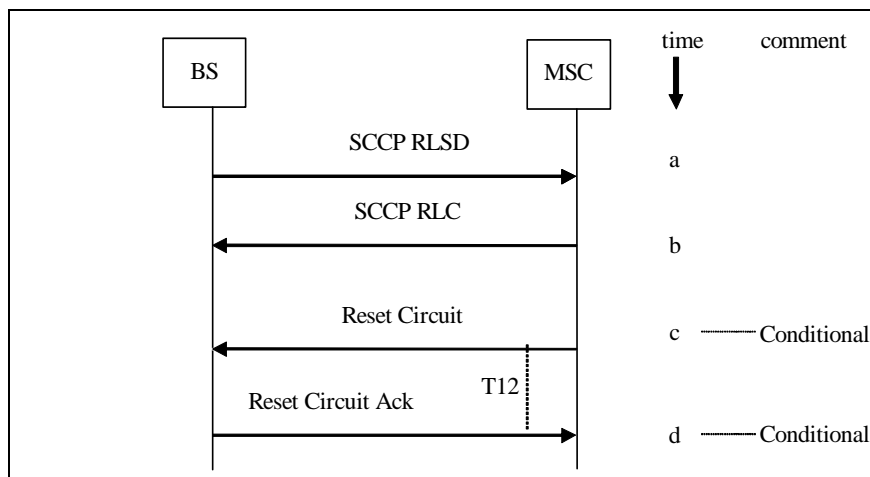
28 Figure 3.1.3.4.3.1-1 BS Initiated SCCP Release: BS Lost SCCP Connection Information
