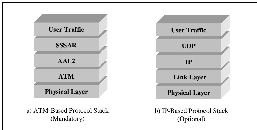
8 Figure 3.3.2-1 A3 User Traffic Protocol Stack
